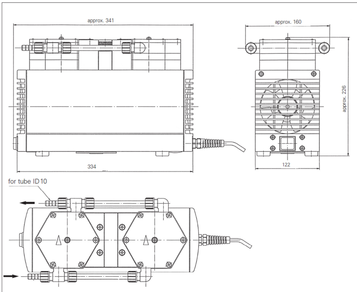
Dimensions (mm)
